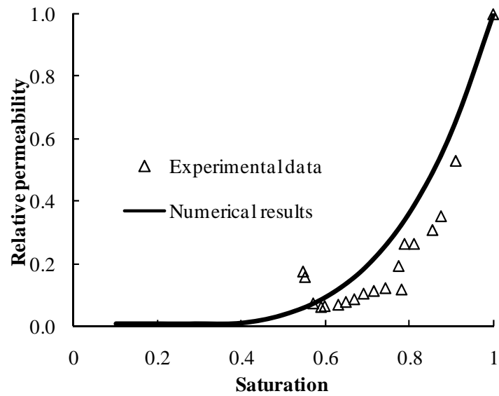
Fig. 11 Variation of relative permeability in function of saturation degree.
