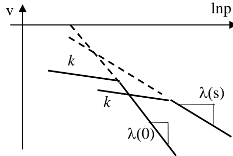
Fig. 8 Compression curve for saturated and unsaturated soil.
