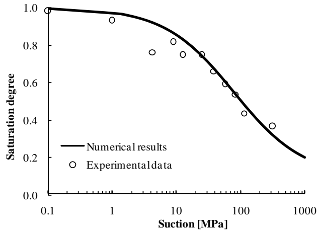
Fig. 10 Water retention curve of GMZ bentonite.
