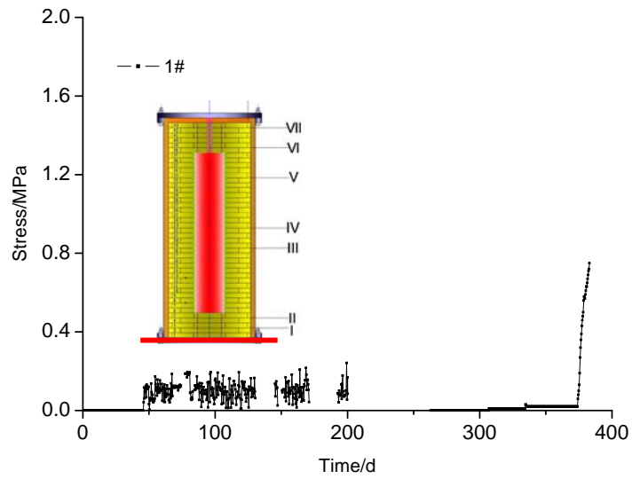
Fig. 6 Stress evolution at the bottom of China-Mock-up.
