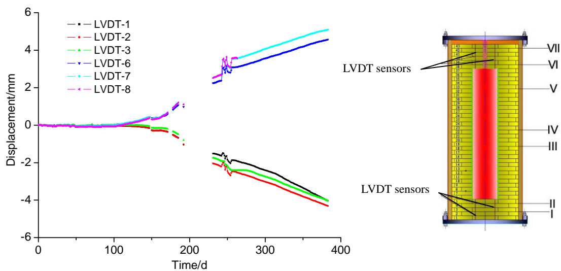
Fig. 5 Vertical displacement of the heater with time.
