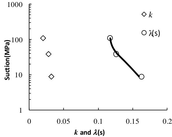
Fig. 13 Variation of k and \lambda(s) with suction.
