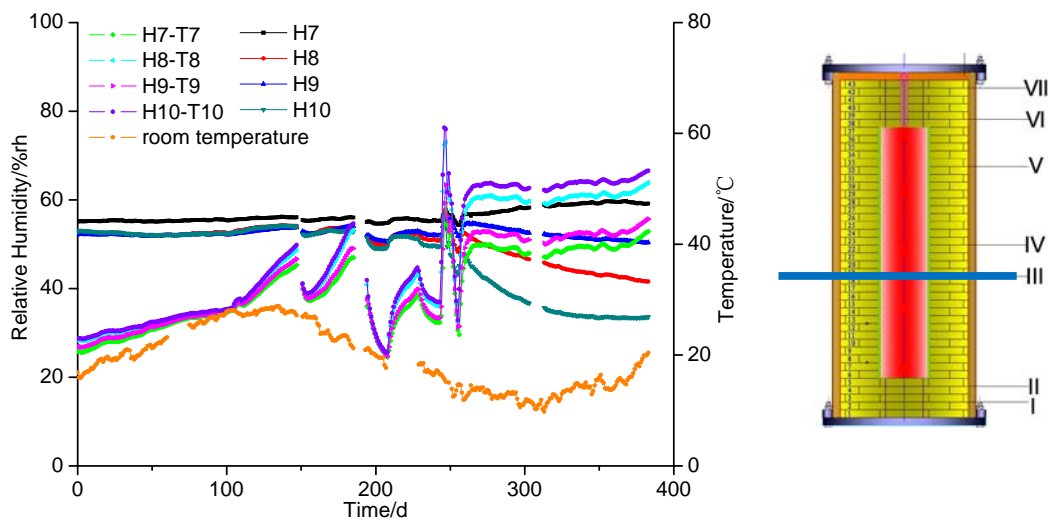
Fig. 4 Relative humidity distribution at section III.
