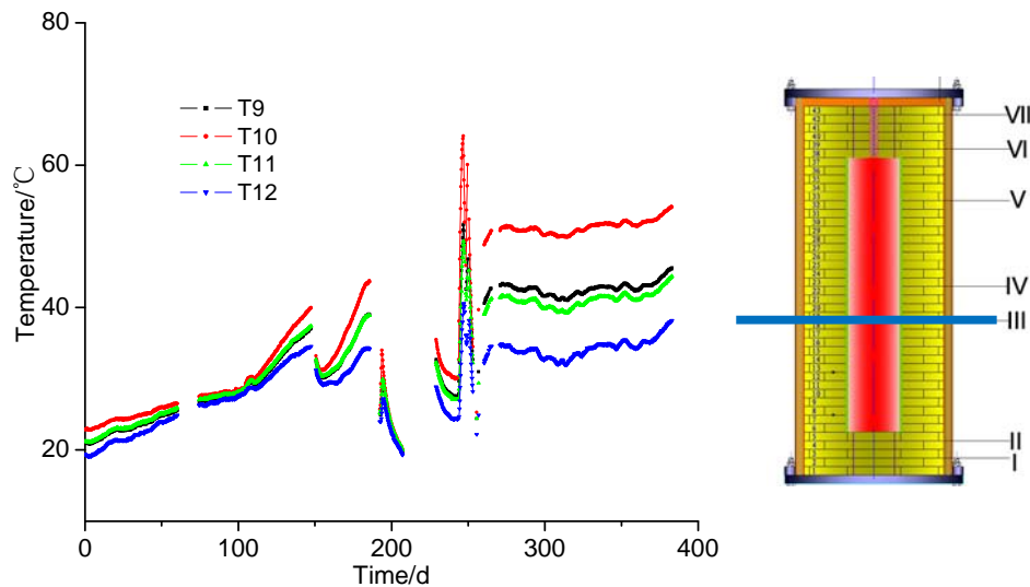
Fig. 2 Temperature variation with time at section III.
