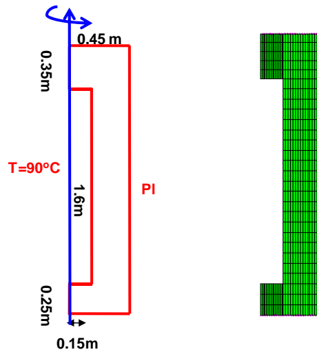
Fig. 9 Boundary conditions and mesh.
