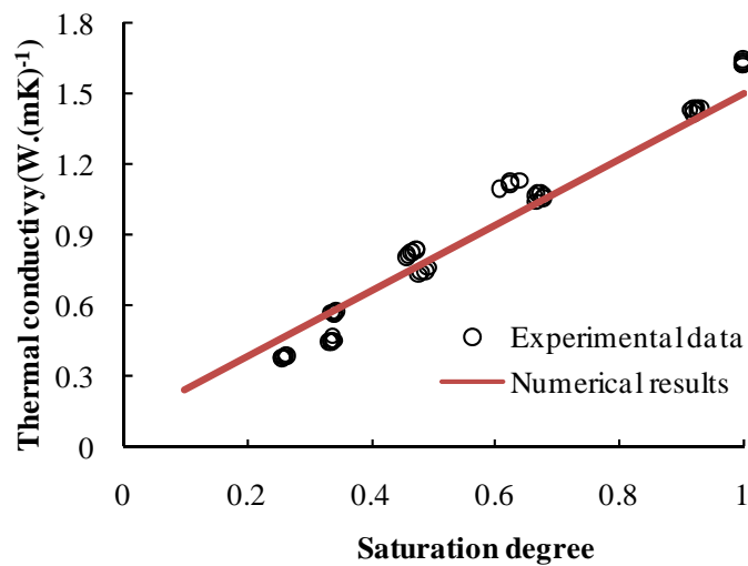
Fig. 12 Variation of thermal conductivity with saturation degree.
