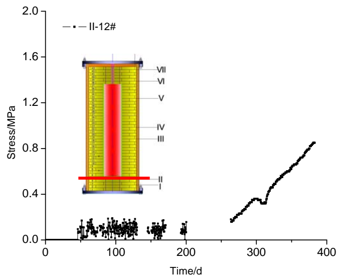
Fig. 7 Stress evolution at section II.
