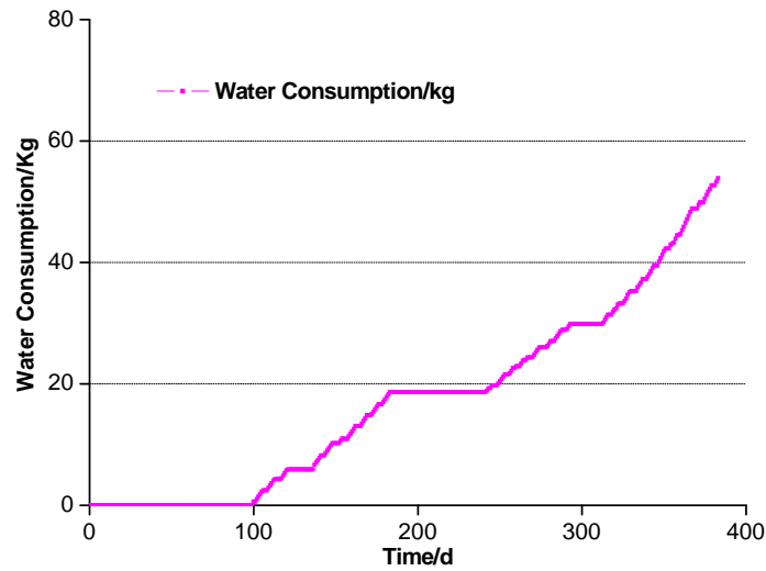
Fig. 3 Water consumption with the time.
