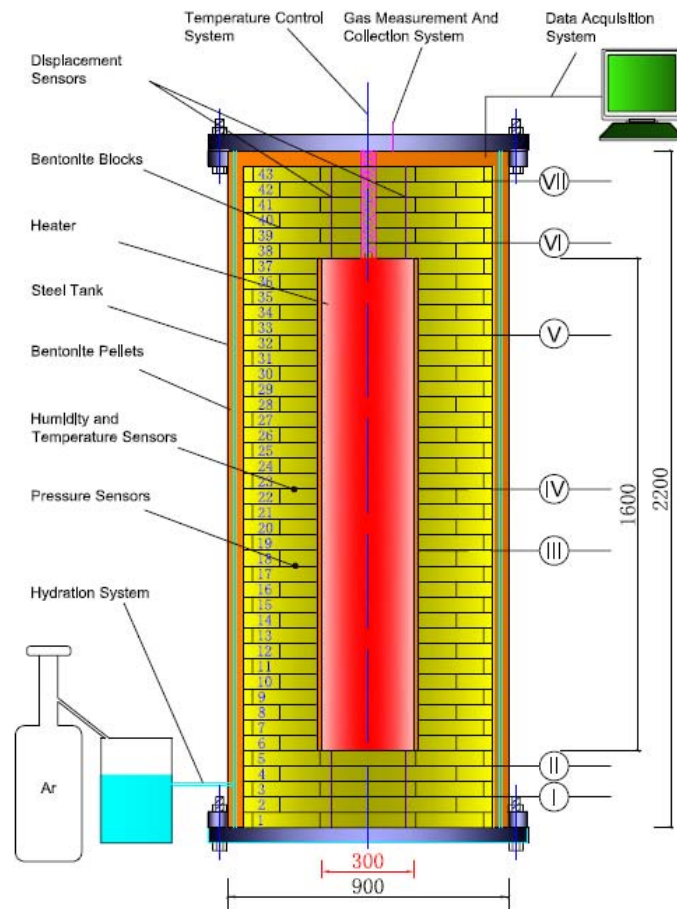
Fig. 1 Sketch of the China-Mock-up facility (unit: mm).
