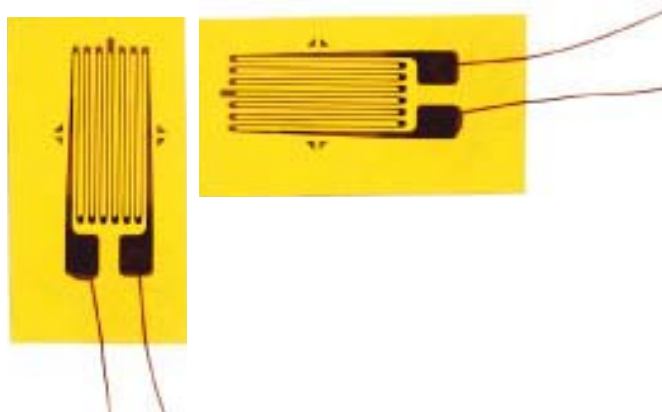
Fig. 14 Resistance strain gauges.
