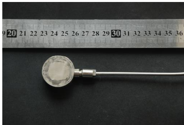
Fig. 9 Hydraulic pressure sensor.
