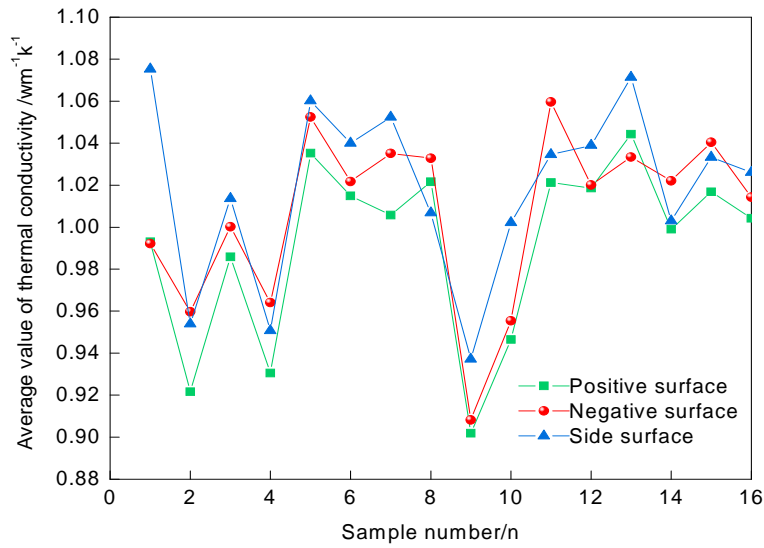
Fig. 6 Distribution of thermal conductivity on different measurement surfaces.
