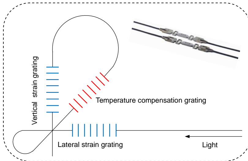
Fig. 13 Fiber Bragg grating (FBG) strain/temperature sensor.
