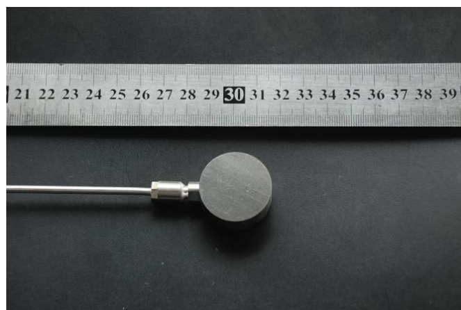
Fig. 8 Stress sensor.
