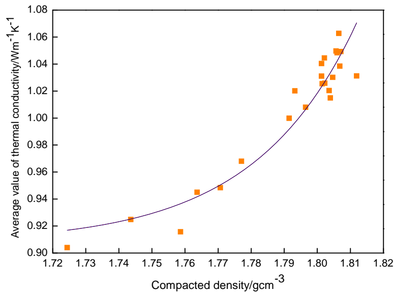
Fig. 7 Relationship between thermal conductivity and compacted density of the bentonite blocks.
